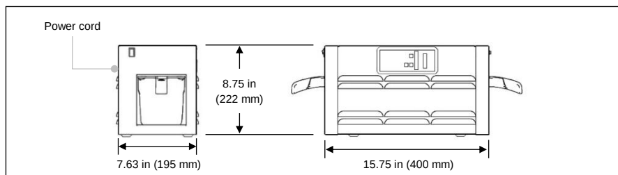
MPC 21L dual access modular multi-purpose holding cabinet
