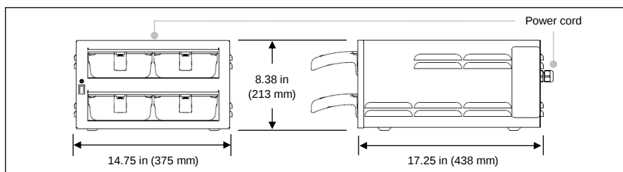
MPC 22 modular multi-purpose holding cabinet
